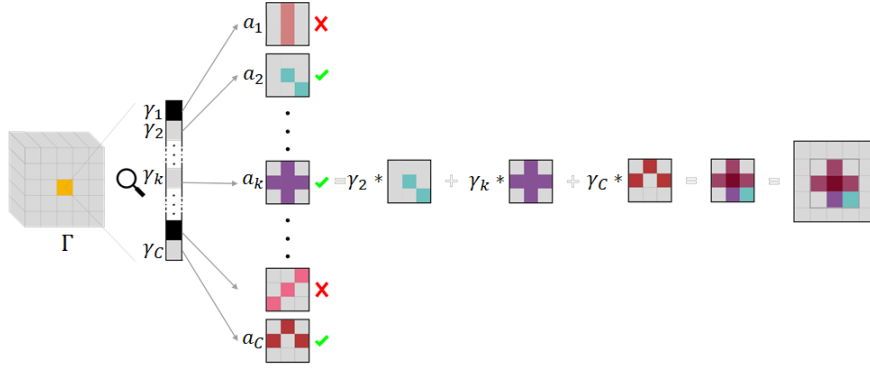
Figure 2: 2D CSC visualization: \Gamma is an H \times W \times C tensor, composed of H \times W “needles”, denoted as \gamma_i , each of size 1 \times 1 \times C . Since \Gamma is sparse, the bulk of its entries is zeros. A given \gamma_i at location i; j in \Gamma contributes to a patch located in the corresponding location in the output image X . Each non-zero entry \gamma_i in \Gamma defines the coefficient for the filter a_i in a superposition that creates a patch. Note that the patches created by nearby needles may overlap, depending on the stride and the spatial size of the atoms in \mathbf{D} .
